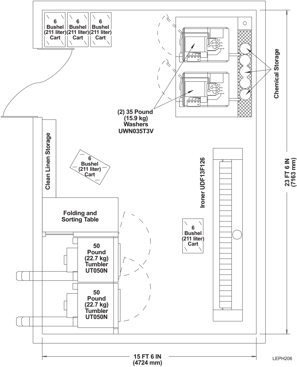
Typical Laundry with Ironer for Flatgoods Capable of Producing 105 Pounds (48 kg) Per Hour (364.3 Square Feet [33.8 Square Meters])
