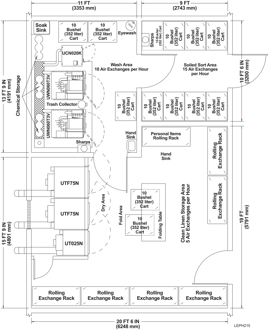
Typical Laundry for a Nursing Home Capable of Producing 166 Pounds (75 kg) Per Hour at 1.2 Loads Per Hour (604.8 Square Feet [56 Square Meters])
