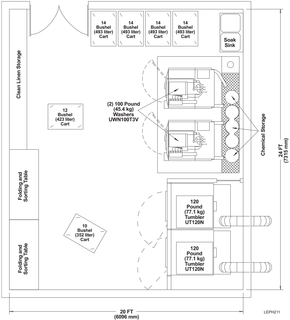
Typical Laundry for No-Iron Linen Capable of Producing 300 Pounds (136 kg) Per Hour (480 Square Feet [44.6 Square Meters])
