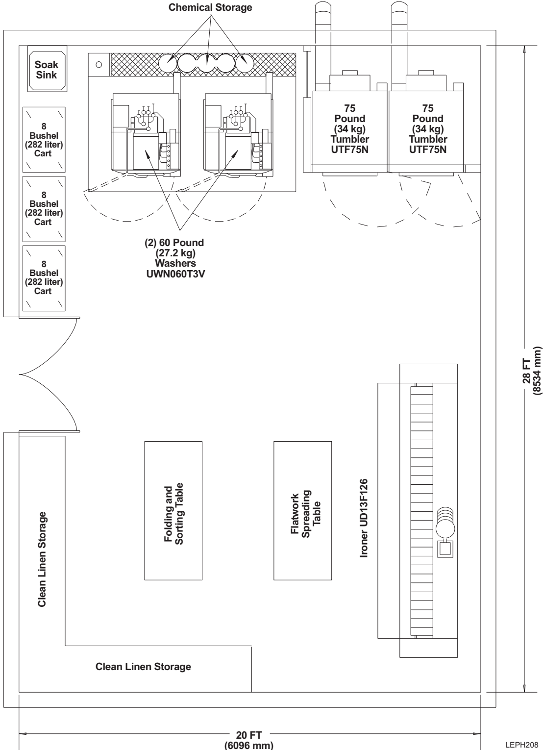
Typical Laundry with Ironer for Flatgoods Capable of Producing 180 Pounds (82 kg) Per Hour (560 Square Feet [52.0 Square Meters])
