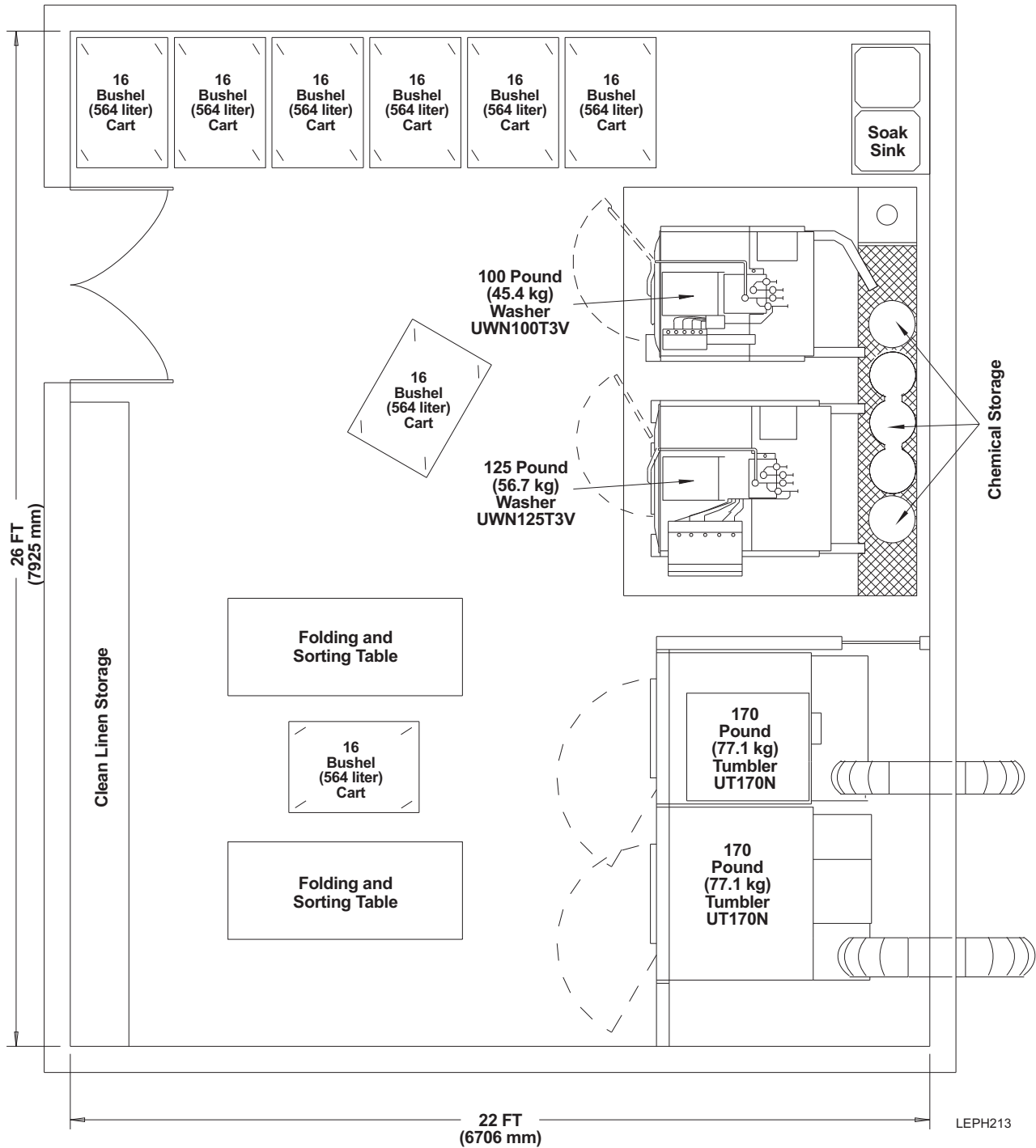
Typical Laundry for No-Iron Linen Capable of Producing 337 Pounds (153 kg) Per Hour (572 Square Feet [53.1 Square Meters])
