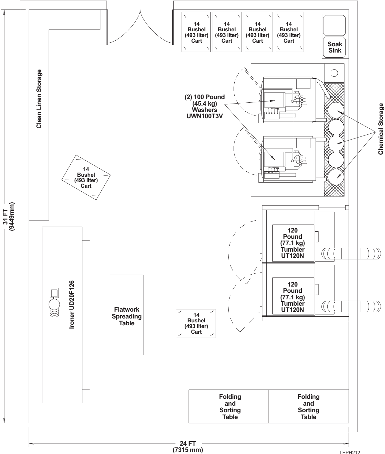
Typical Laundry with Ironer for Flatgoods Capable of Producing 300 Pounds (136 kg) Per Hour (744 Square Feet [69.1 Square Meters])
