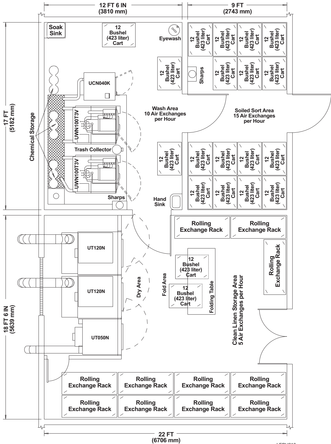
Typical Laundry for a Nursing Home Capable of Producing 282 Pounds (128 kg) Per Hour at 1.2 Loads Per Hour (781 Square Feet [72.5 Square Meters])
