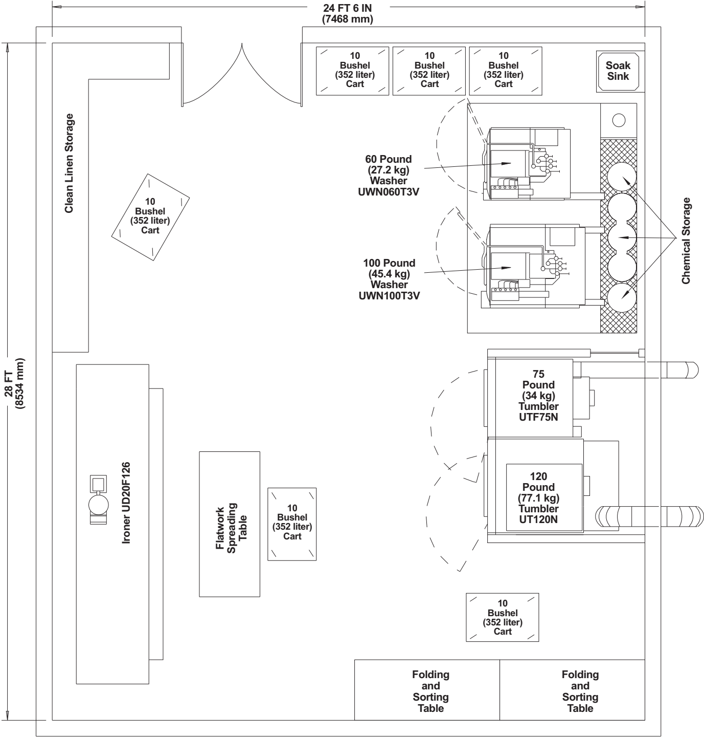
Typical Laundry with Ironer for Flatgoods Capable of Producing 240 Pounds (109 kg) Per Hour (686 Square Feet [63.7 Square Meters])
