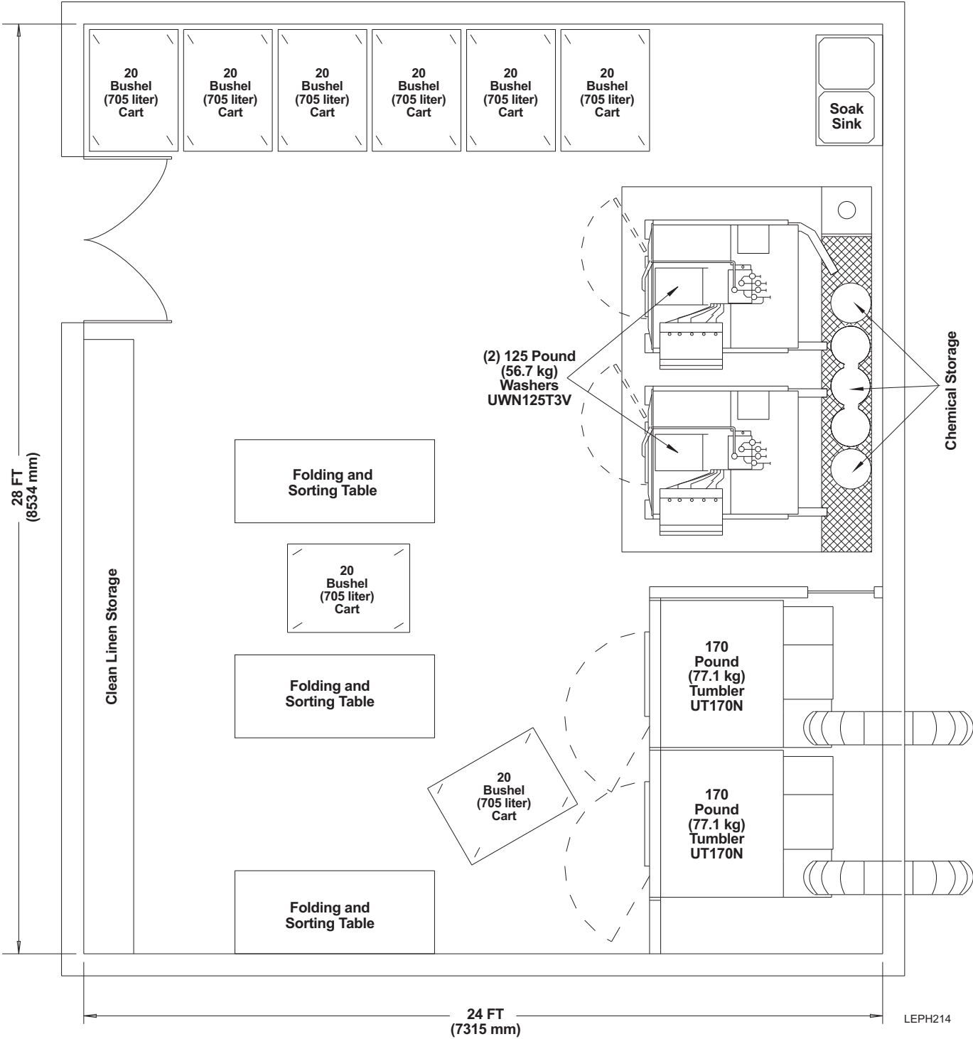
Typical Laundry for No-Iron Linen Capable of Producing 375 Pounds (170 kg) Per Hour (672 Square Feet [62.4 Square Meters])
